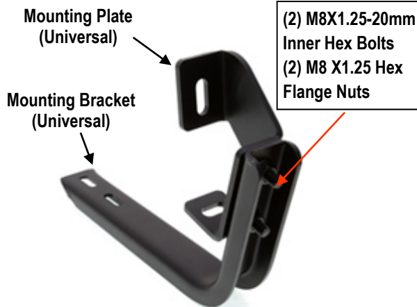
(Fig 6) Driver Front Mounting Bracket Assembled
