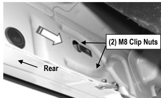
(Fig 5) Driver Rear Mounting Bracket Location
