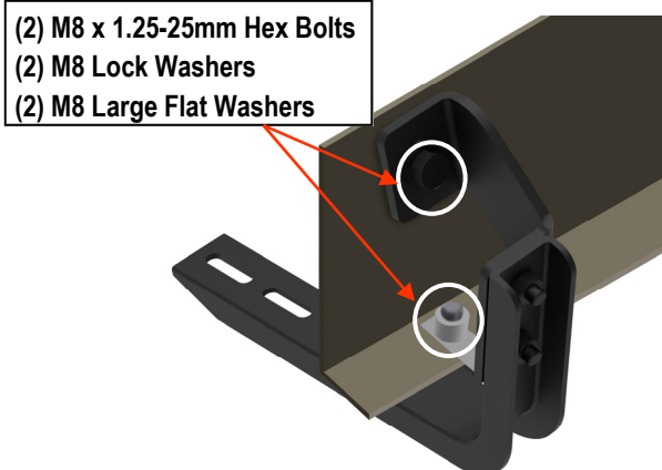
(Fig 7) Assembled Driver Front Bracket Installed
